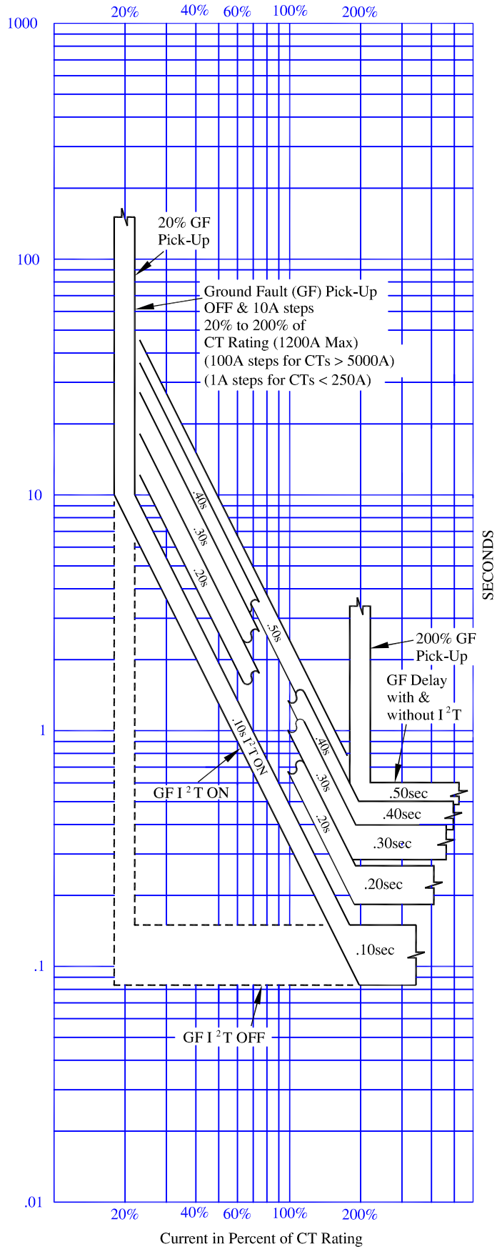
Ground Fault Time Current Curve
