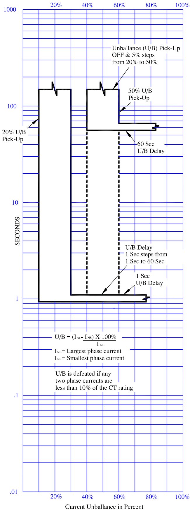
Unbalance Time Current Curve
