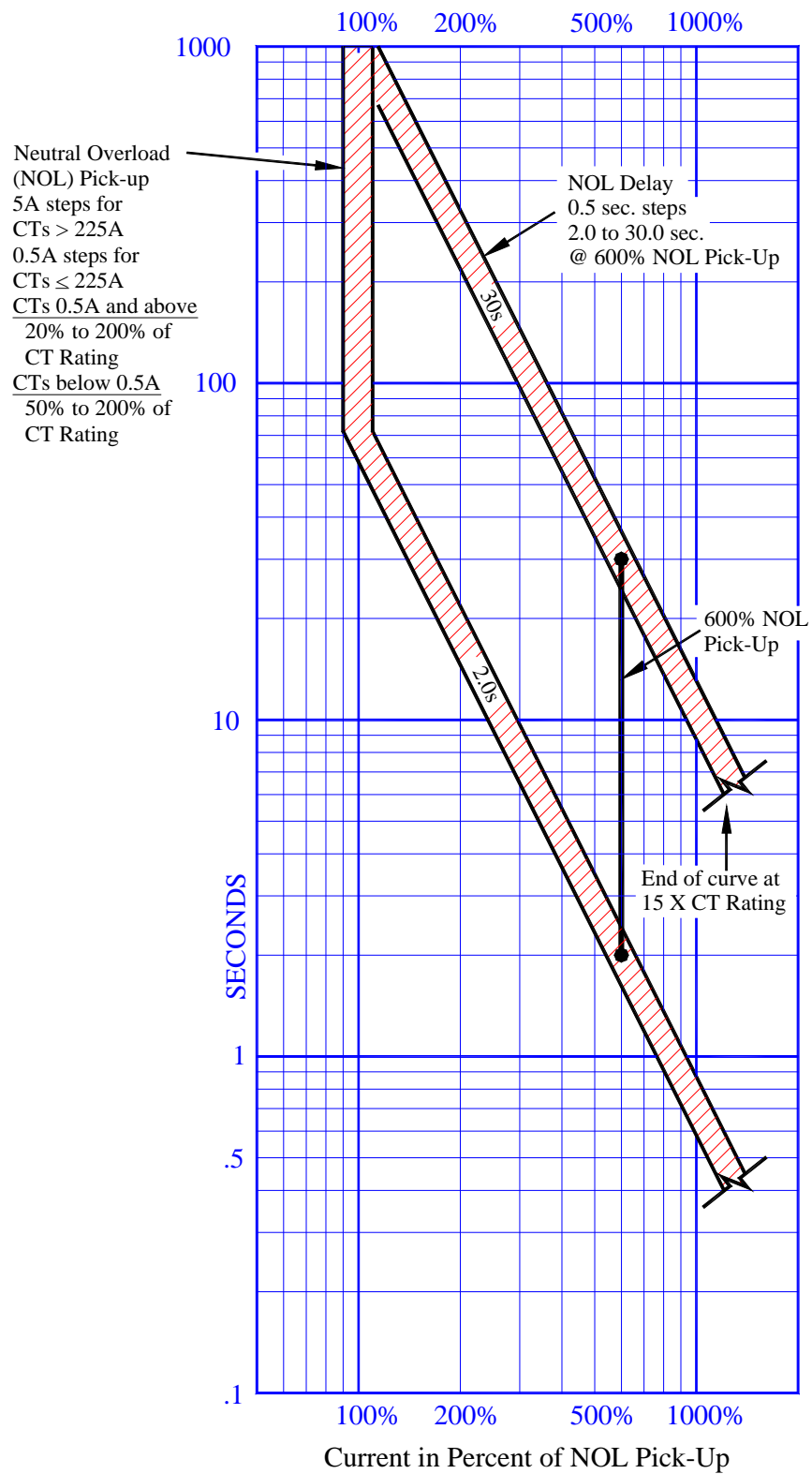
Figure 15: AC-PRO-II Neutral Overload TCC
