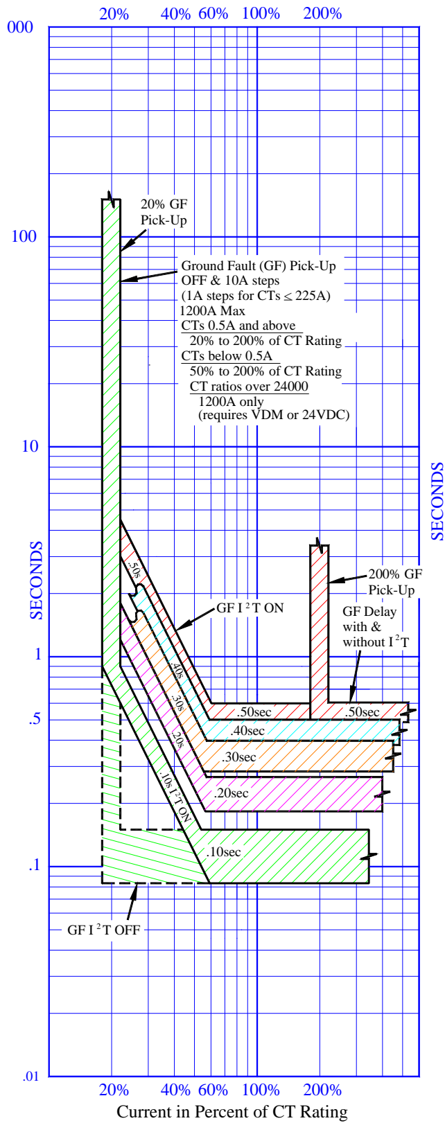
Figure 13: AC-PRO-II Ground Fault TCC
