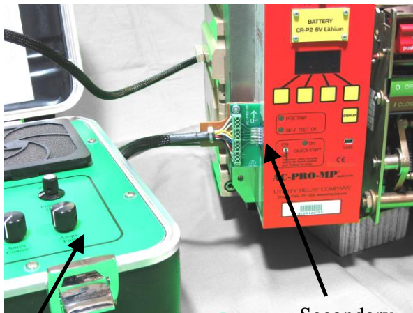
Secondary injection test set
